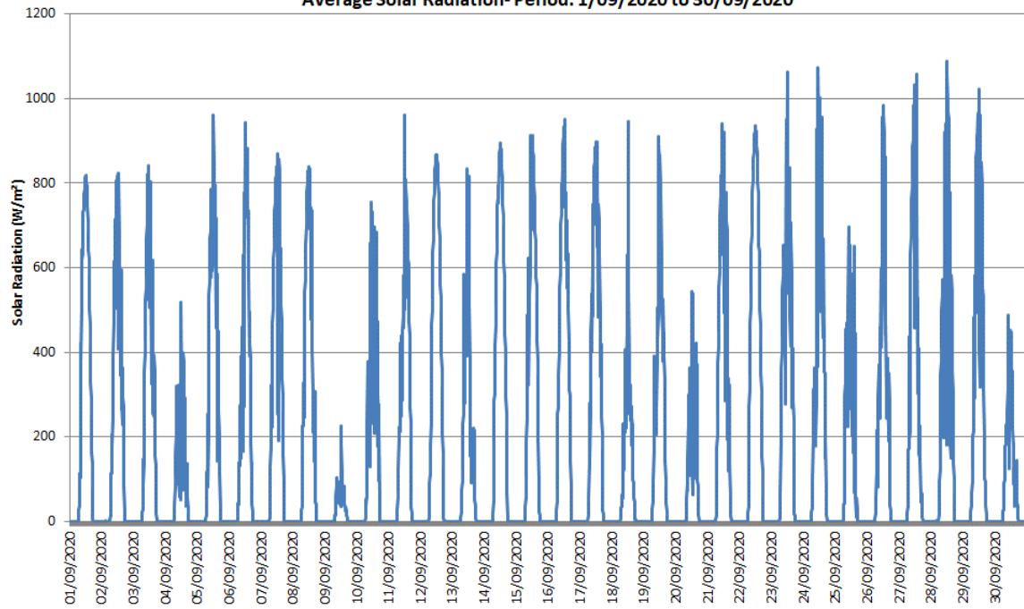
Blackmans Flat NSW Average Solar Radiation- Period: 1/09/2020 to 30/09/2020
